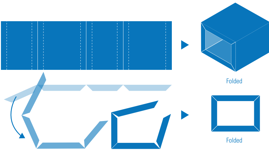
Modern Miter Folding — OMNOVA Laminates (2 piece assembly)
